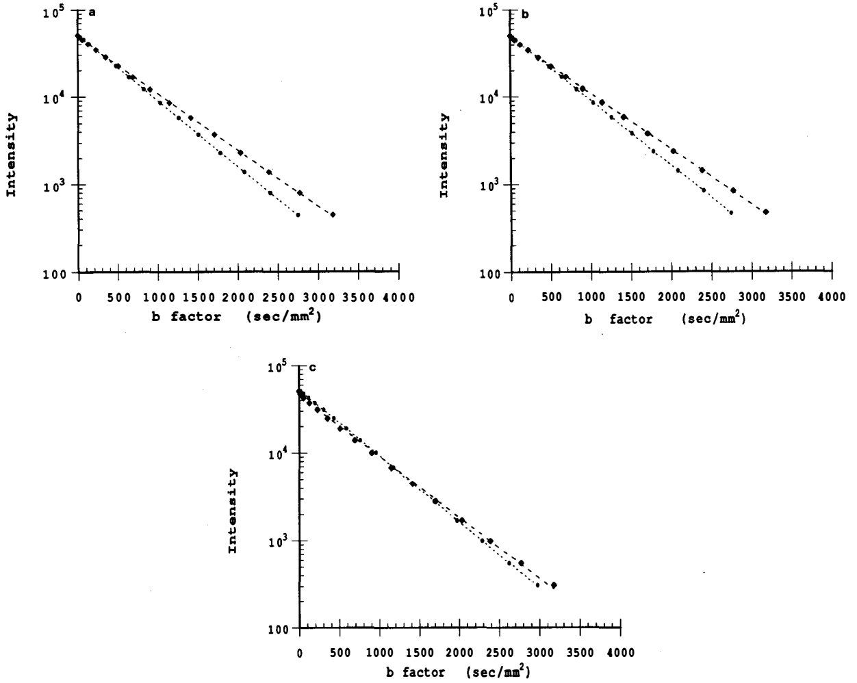
FIG. 4. The signal intensity versus the diagonal b matrix for the three directions (read, phase, and slice) for the water phantom: (a) x direction (phase), (b) y direction (slice), and (c) z direction (read). Using Eqs. [11], [12], and [13], we see that both the goodness of fit and the agreement with the diffusivities estimated from imaging and spectroscopic measurements indicate that the b -matrix values were calculated correctly (●). To demonstrate the effect of cross terms on the estimation of the diffusivity, we also calculated the scalar b factors using Eq. [9], intentionally omitting the cross terms (◆). Both the poor fit and the significant disagreement with the diffusivity estimated from spectroscopic measurements demonstrate that calculating the b factors without the cross terms leads to significant errors in the estimation of diffusivities.
