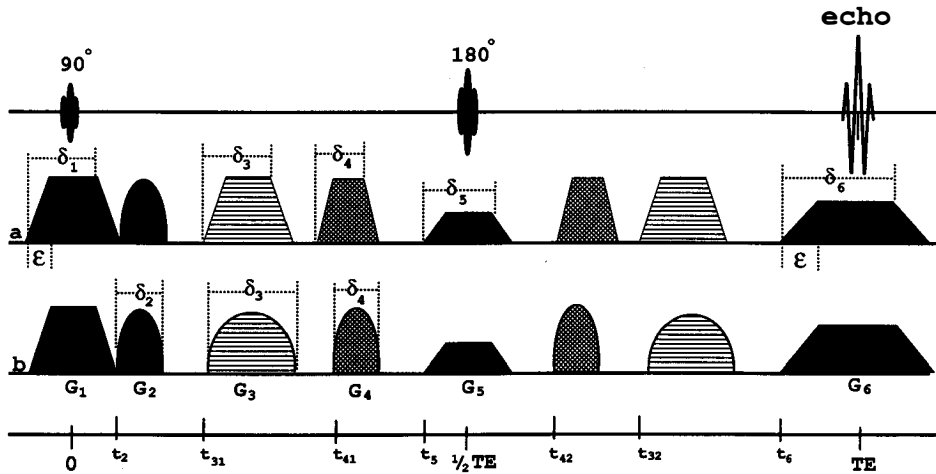
FIG. 2. The generalized imaging gradient-pulse sequences used to derive the analytical b -matrix expressions. In this figure G_{ki} ( k = 1 through 6) are the gradient-pulse strengths in the i th coordinate direction (i.e., the read, phase, or slice direction). The different gradients are G_1 , the 90^\circ slice-selection gradient; G_2 , a phase-encode, read-dephase, or slice-refocusing gradient; G_3 , a diffusion gradient; G_4 , a crusher gradient; G_5 , the 180^\circ slice-selection gradient; and G_6 , the readout gradient. \delta_k is the pulse duration, \epsilon is the rise time of the trapezoidal ramp, and t_k is the time at which the gradient pulse turns on. In this figure, gradient pulses are shown with (a) trapezoidal or (b) sinusoidal diffusion and crusher gradients.
