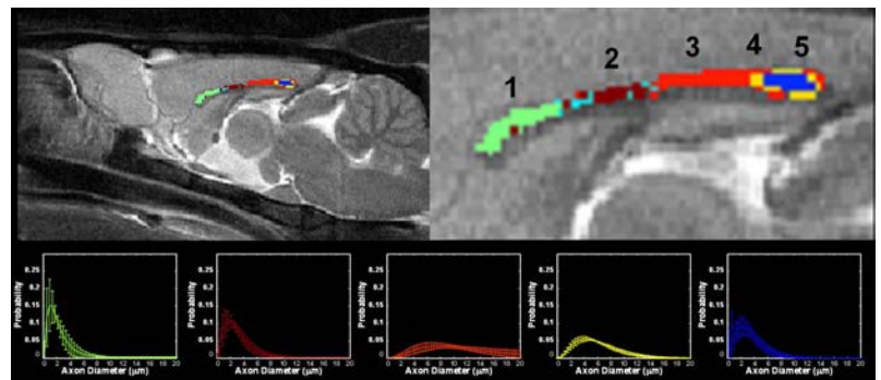
Figure 1: Cluster analysis of the ADD in the rat CC measured in-vivo estimated from AxCaliber. The different colors represents distinct clusters found by the k-means algorithm with the corresponding the ADD shown in the graphs.
